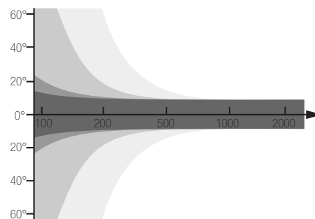
Vertical directivity from 100 Hz to 2 kHz from light grey to dark grey respectively with 1x ID84, 2x ID84, 2x ID84 + 1x ID84L and 2x ID84 + 2x ID84L line.
