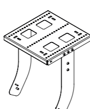
VNI-VCPL425 (ePS8 under eLS600) VNI-HCPL535 (ePS10 under eLS600) VNI-VCPL365 (ePS6 under eLS400) VNI-HCPL425 (ePS8 under eLS400) VNI-HCPL600 (ePS12 under eLS18) VNI-HCPL535 (ePS10 under eLS600) eLS and ePS clusters
