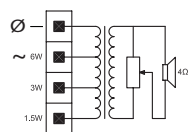
Circuit diagram LB1-UW06V-x
