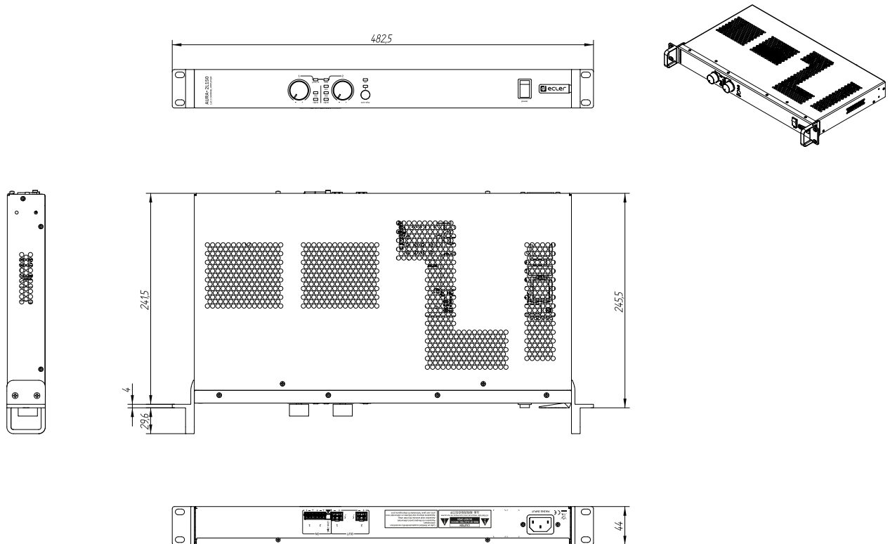
Ecler AURA-2L150 Mechanical Diagram
