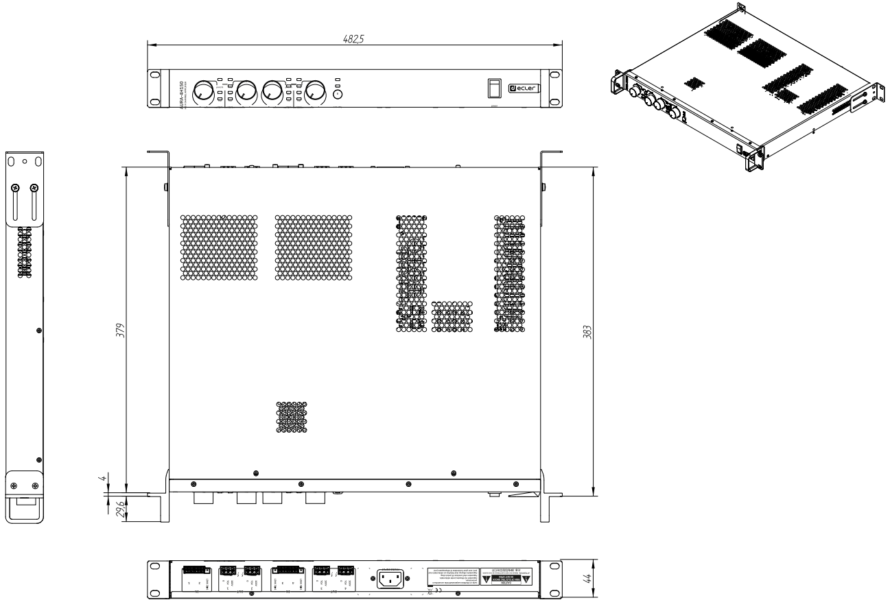
Ecler AURA-4HI150 Mechanical Diagram
